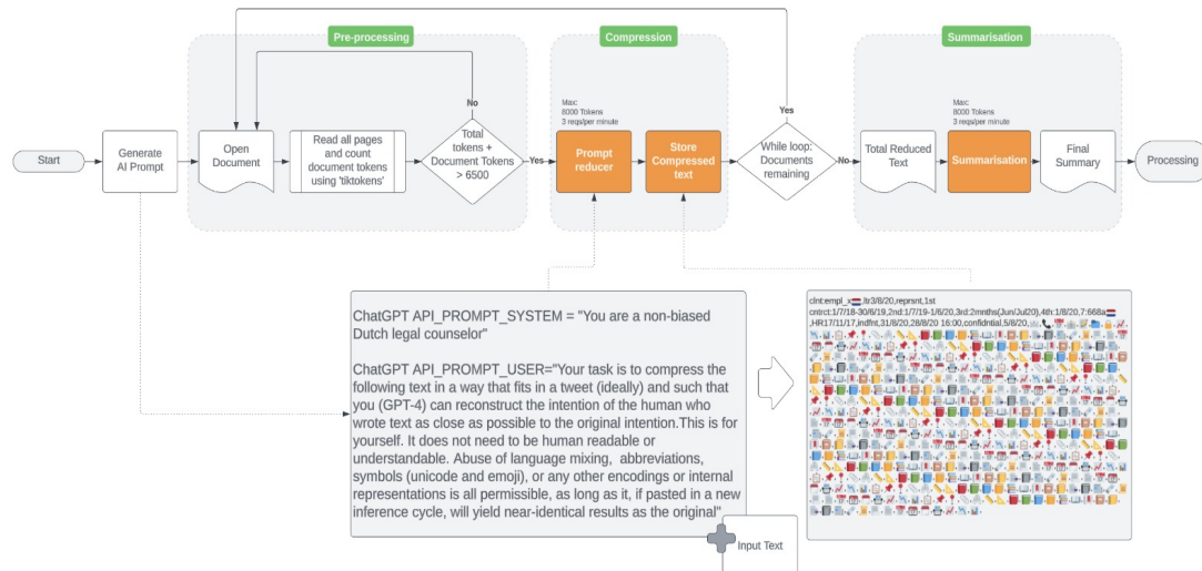
Figure 4: Pre-processing and compression process
