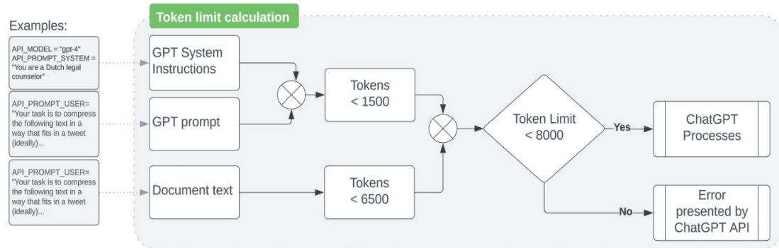
Figure 3: Token limit calculation
